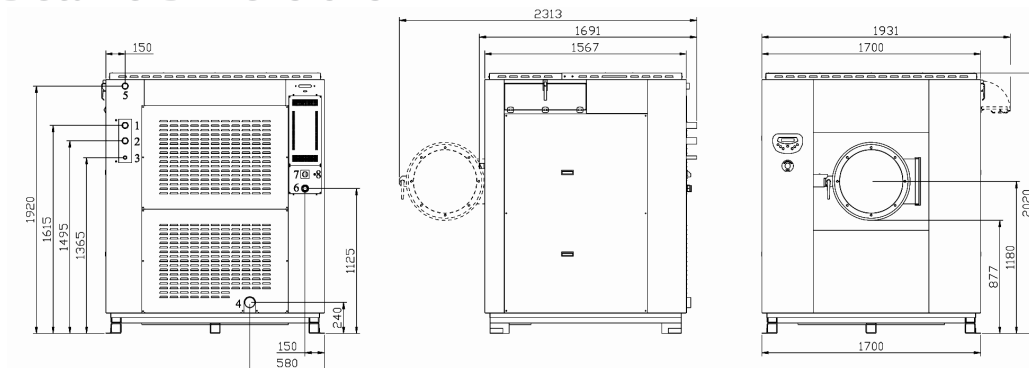
MACHINE FRONT
