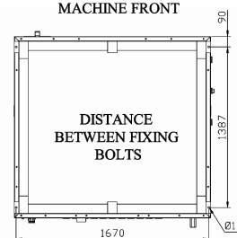
MACHINE FRONT
