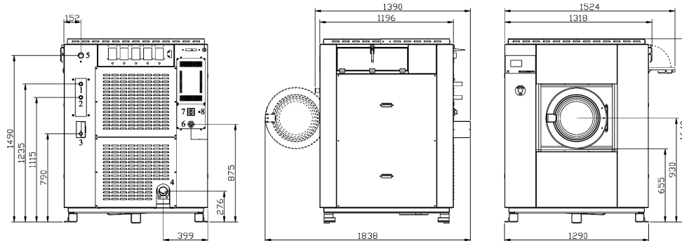
MACHINE FRONT
